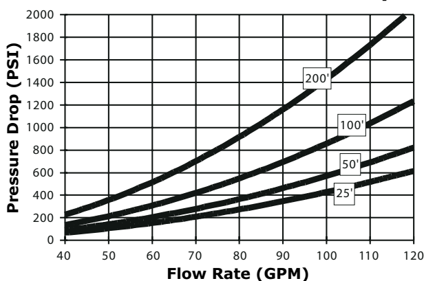
20mm Hose Pressure Drop
